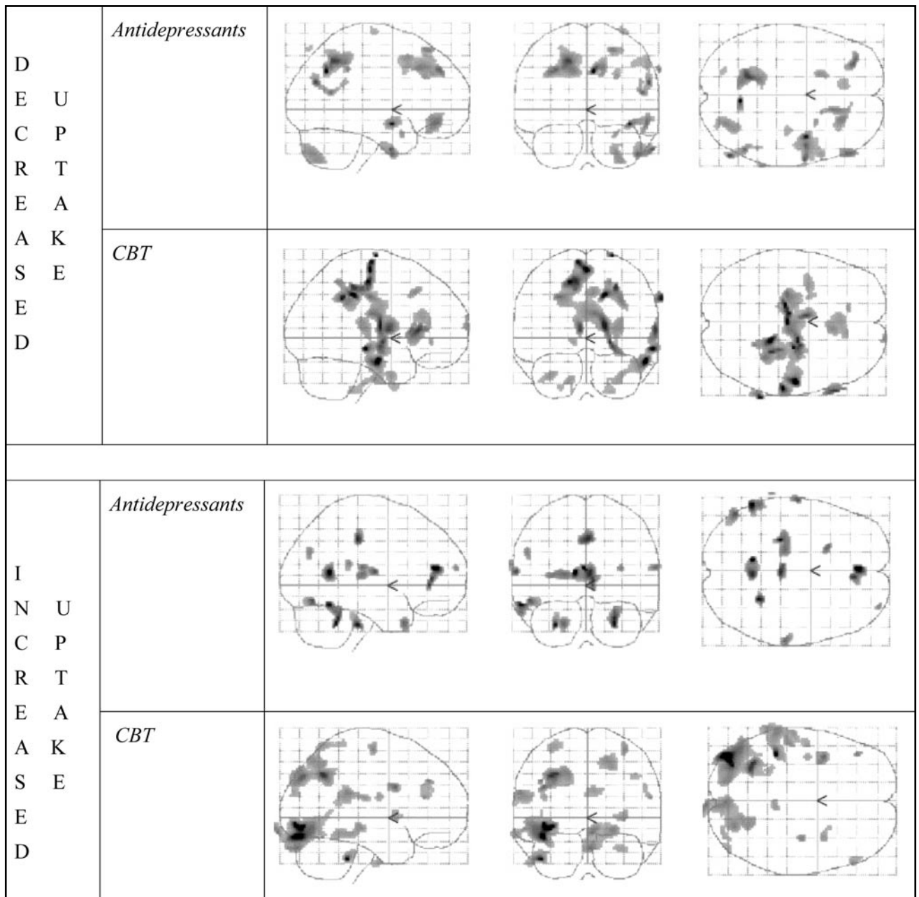
Figure 4: Regions of decreased and increased 18 FDG-PET uptake in the group of patients treated with antidepressants or CBT.
